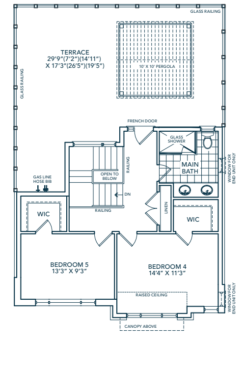
OPTIONAL THIRD FLOOR WITH BEDROOM 5
