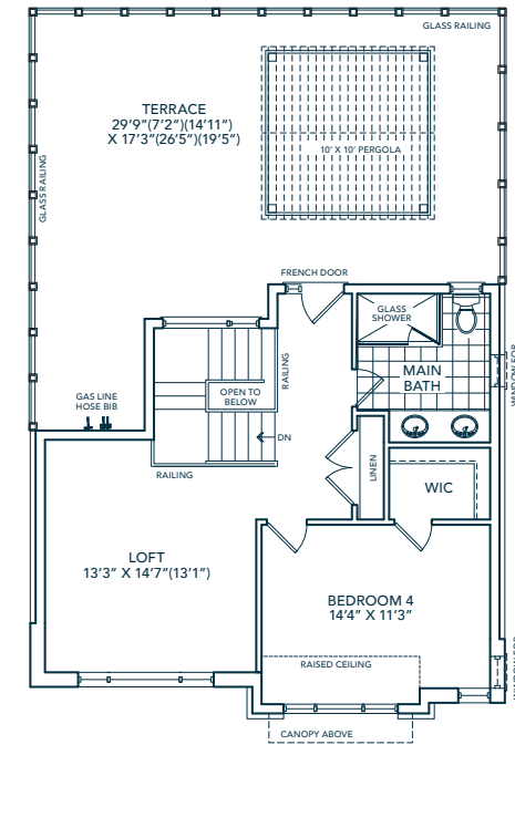
THIRD FLOOR
