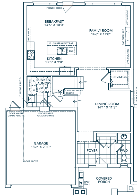
OPTIONAL GROUND FLOOR W/ ELEVATOR
