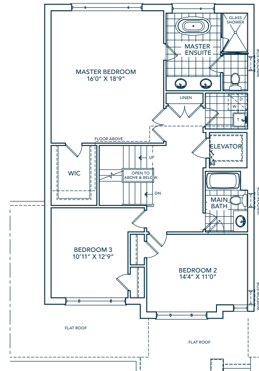
OPTIONAL SECOND FLOOR W/ ELEVATOR
