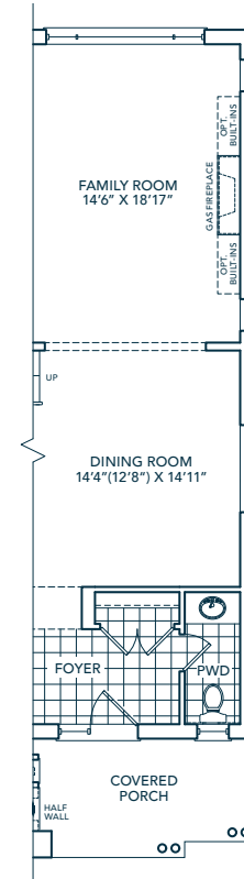
PARTIAL GROUND FLOOR ELEV. B (BLOCK 21)
