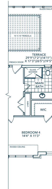
PARTIAL THIRD FLOOR ELEV. A (BLOCK 1)
