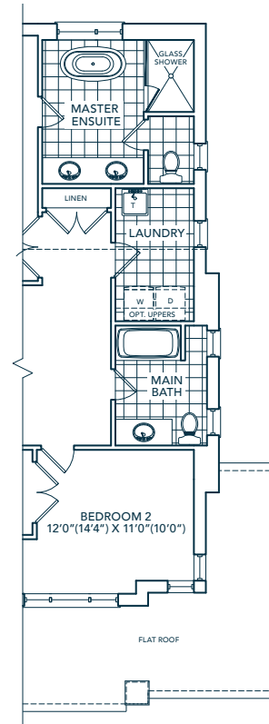
PARTIAL SECOND FLOOR ELEV. A CORNER UPGRADE (BLOCK 13)
