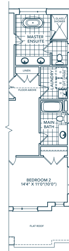
PARTIAL SECOND FLOOR ELEV. B (BLOCK 21)
