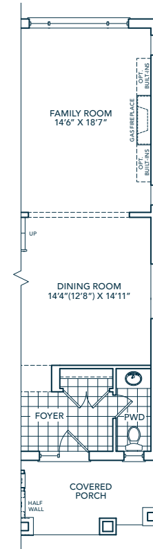
PARTIAL GROUND FLOOR ELEV. A (BLOCK 1)
