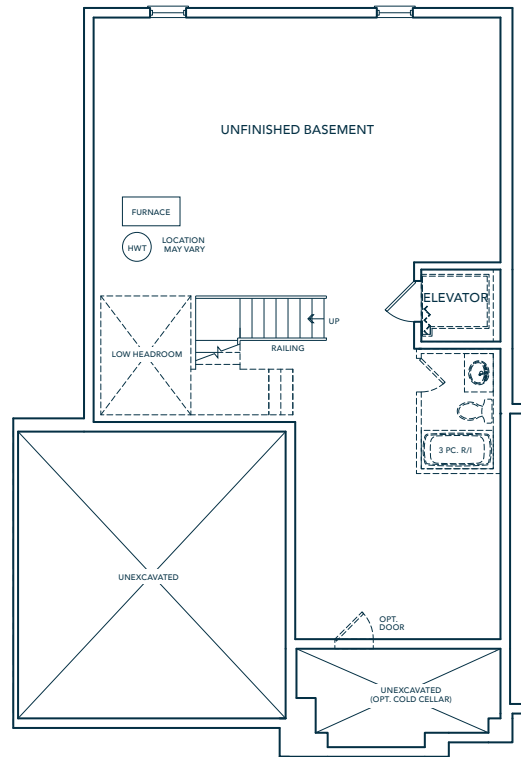
OPTIONAL BASEMENT W/ ELEVATOR
